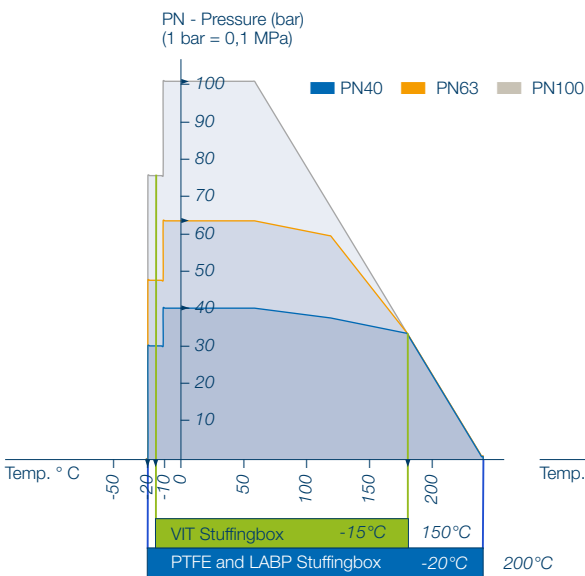
PT diagram for the sealing elements PP
